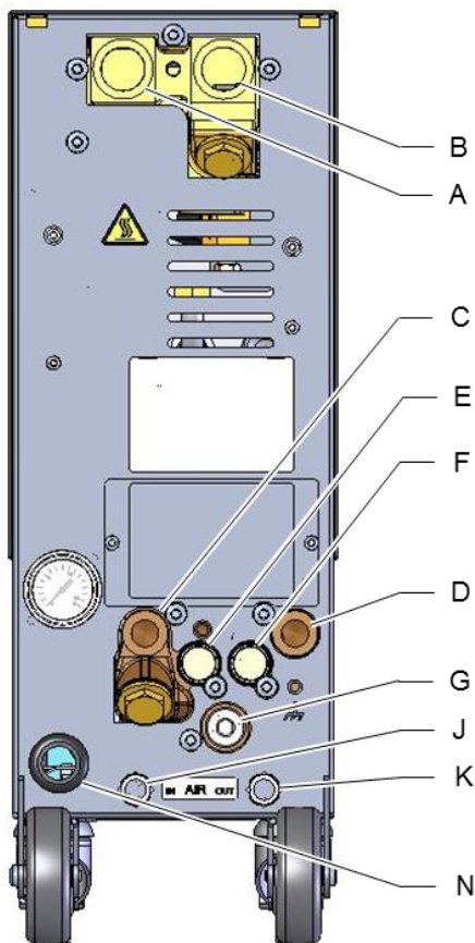
Abb. 5: Anschlüsse
