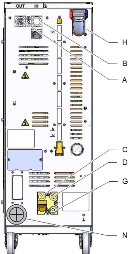
Abb. 5: Anschlüsse
