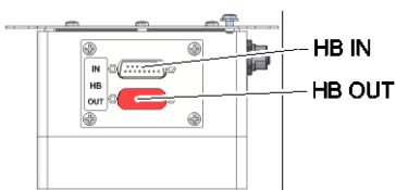
Fig. 16: Interfaces Flow-5 Version : autonome
