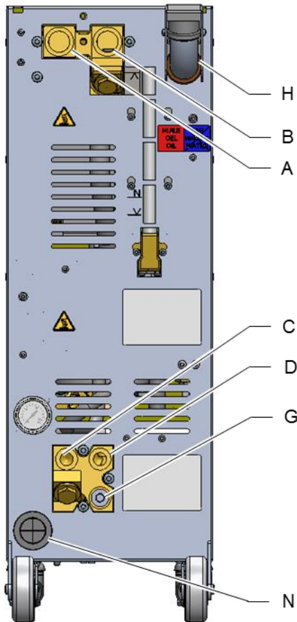
Fig. 5 : Raccordements
