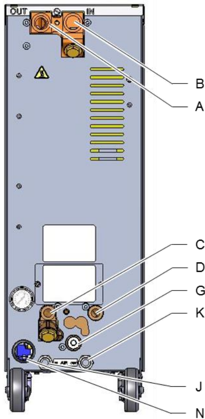
Abb. 5: Anschlüsse
